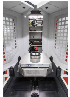
RS 2 robot system
