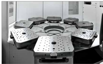
Pallet changer PW 150 8-fold rack storage
